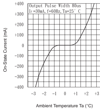
Fig.7 On-State Characteristics
